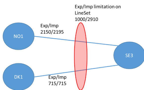
FIGURE 1 PRINCIPLE SKETCH OF THE SE3LS CONCEPT WITH AND EXAMPLE CAPACITY SE3>SE3LS = 1000 MW
